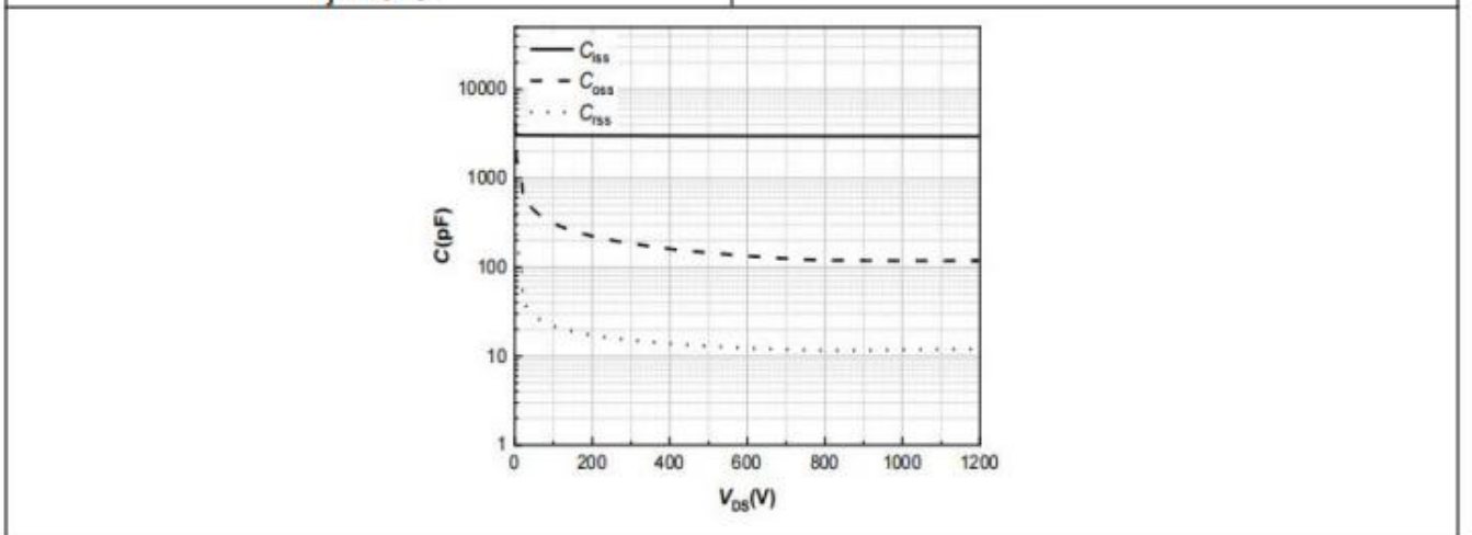
Figure 17. Capacitances vs. Drain-Source
