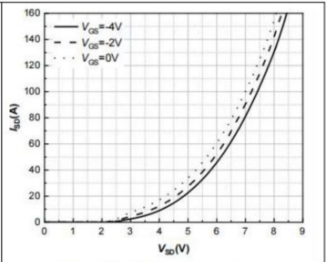
Figure 8. Body Diode Characteristic T_J=-40^{\circ}C
