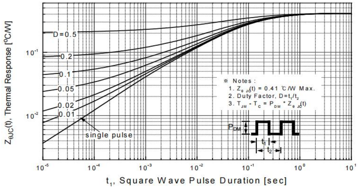
Fig 11: Transient Thermal Response Curve
