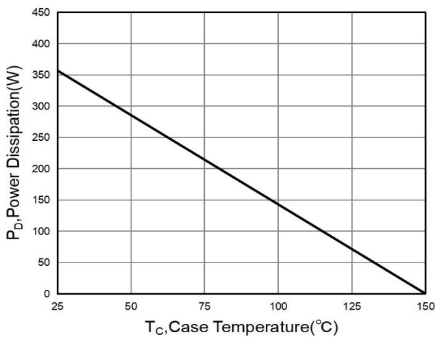
Fig 9: Power Dissipation
